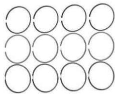
KP-VW-06118 Piston Ring Set 038198151 038 196 189 79.50mm 1.75X2.0X3.0 PASSAT POLO TRANSPORTER SHARAN
